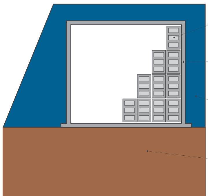
Figure 2. Illustration of multi-barrier vault for low level waste.
